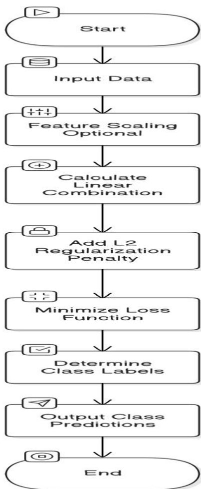
Figure: Ridge Classifier
